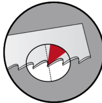
Hook (Positive Rake)
